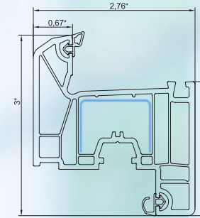
sash
