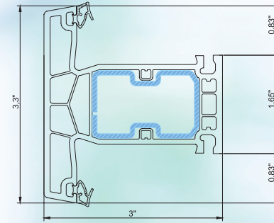
mullion
