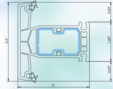
mullion
