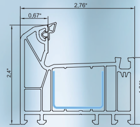
frame
