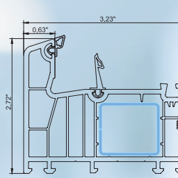
frame
