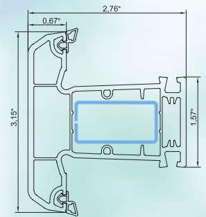
mullion
