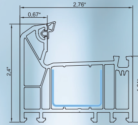
frame
