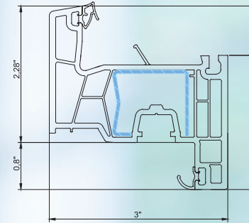
sash
