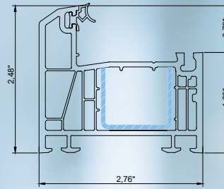
frame
