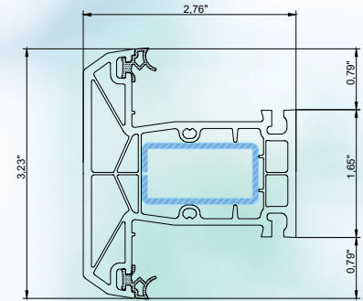
mullion
