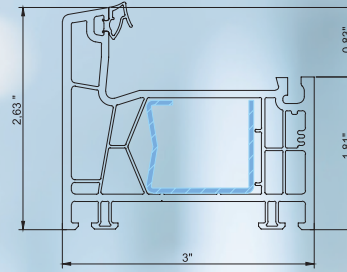
frame
