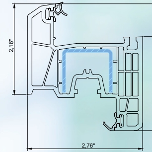
sash
