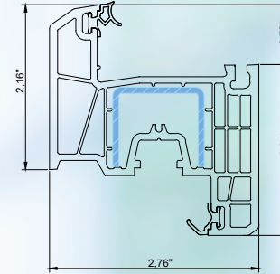
sash
