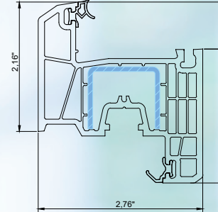
sash
