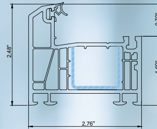
frame
