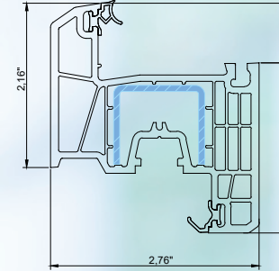
sash
