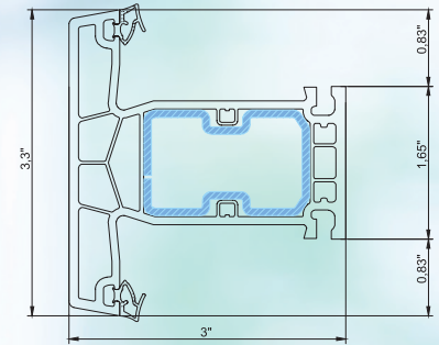
mullion
