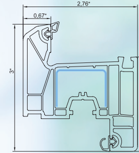
sash
