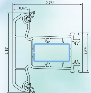
mullion
