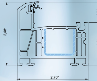
frame
