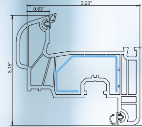
sash
