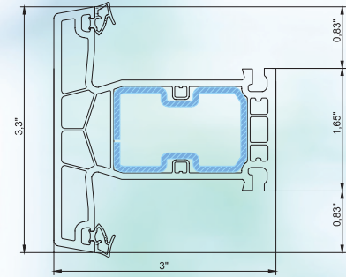
mullion
