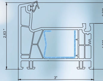
frame
