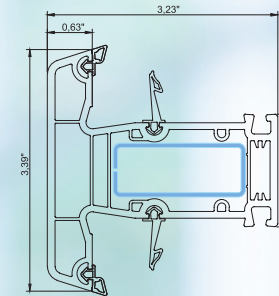
mullion
