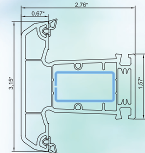
mullion
