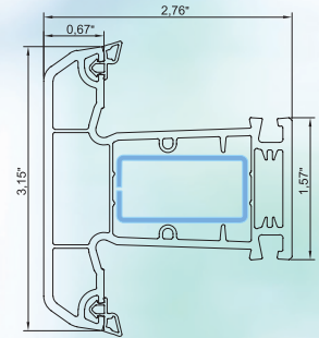
mullion
