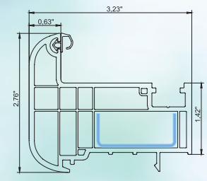
gusset
