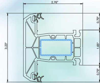
mullion
