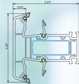
mullion
