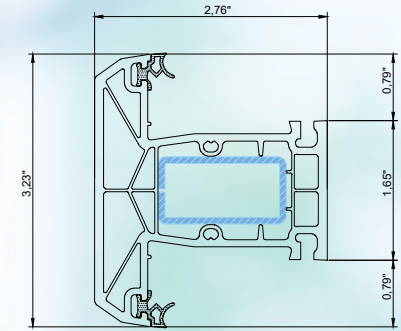
mullion
