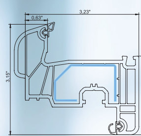
sash
