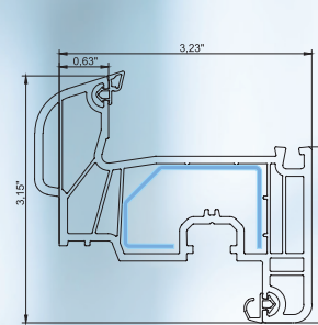
sash
