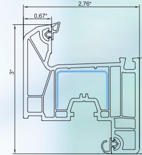
sash
