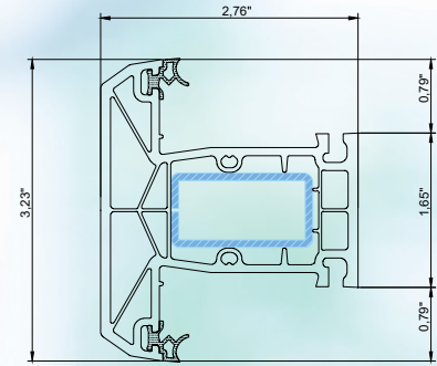
mullion
