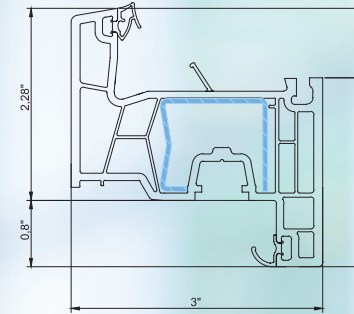
sash
