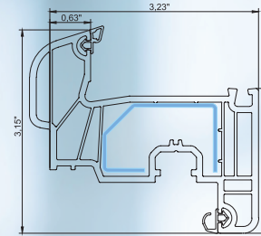
sash
